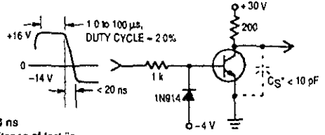
Figure 2. Turn-Off Time
