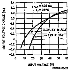
Line Regulation
