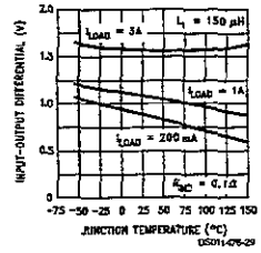
Dropout Voltage
