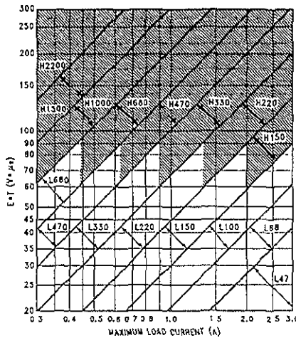
FIGURE 7. LM2576(HV)-ADJ
