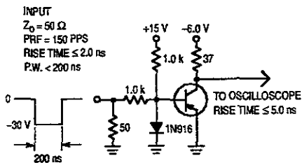
Figure 2. Storage and Fall Time Test Circuit
