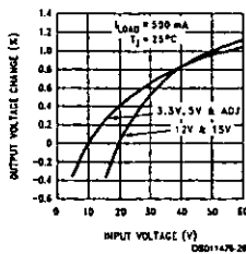
Line Regulation
