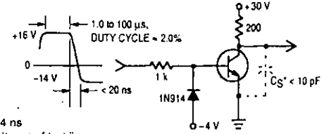
Figure 2. Turn-Off Time
