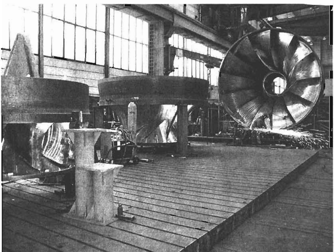
Borca Runner Grinding And Hirakud In Front (Cortesía de Volth Siemens Hydro Power Generation)
