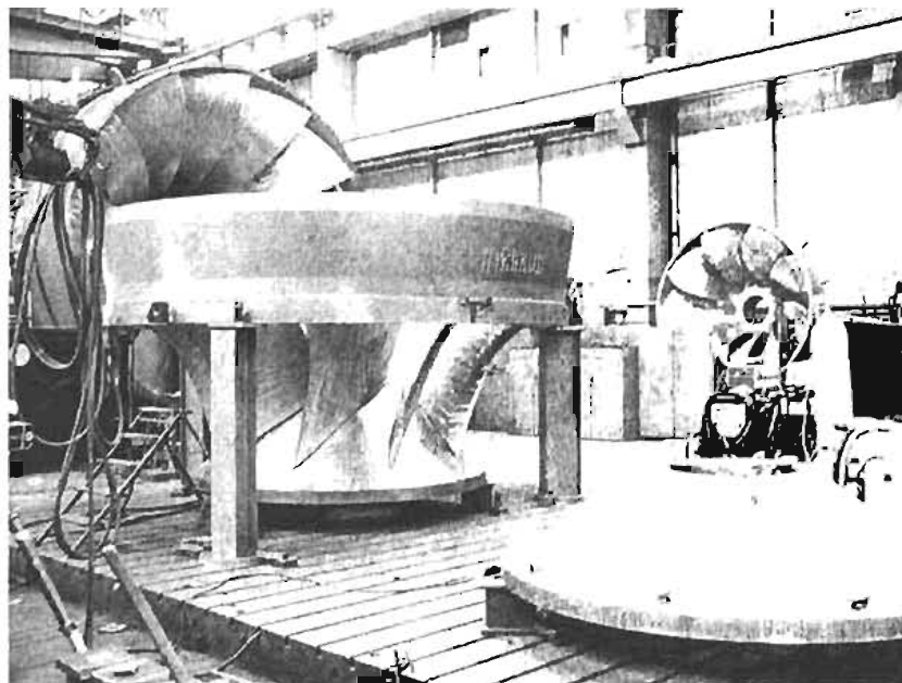
Hirakud Runner Front And In Back Right (Cortesía de Voith Siemens Hydro Power Generation)
